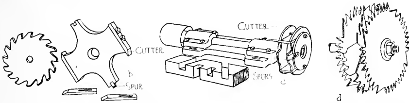
FIG. 173. GROOVING AND GAINING HEADS FOR UNIVERSAL SAW.
